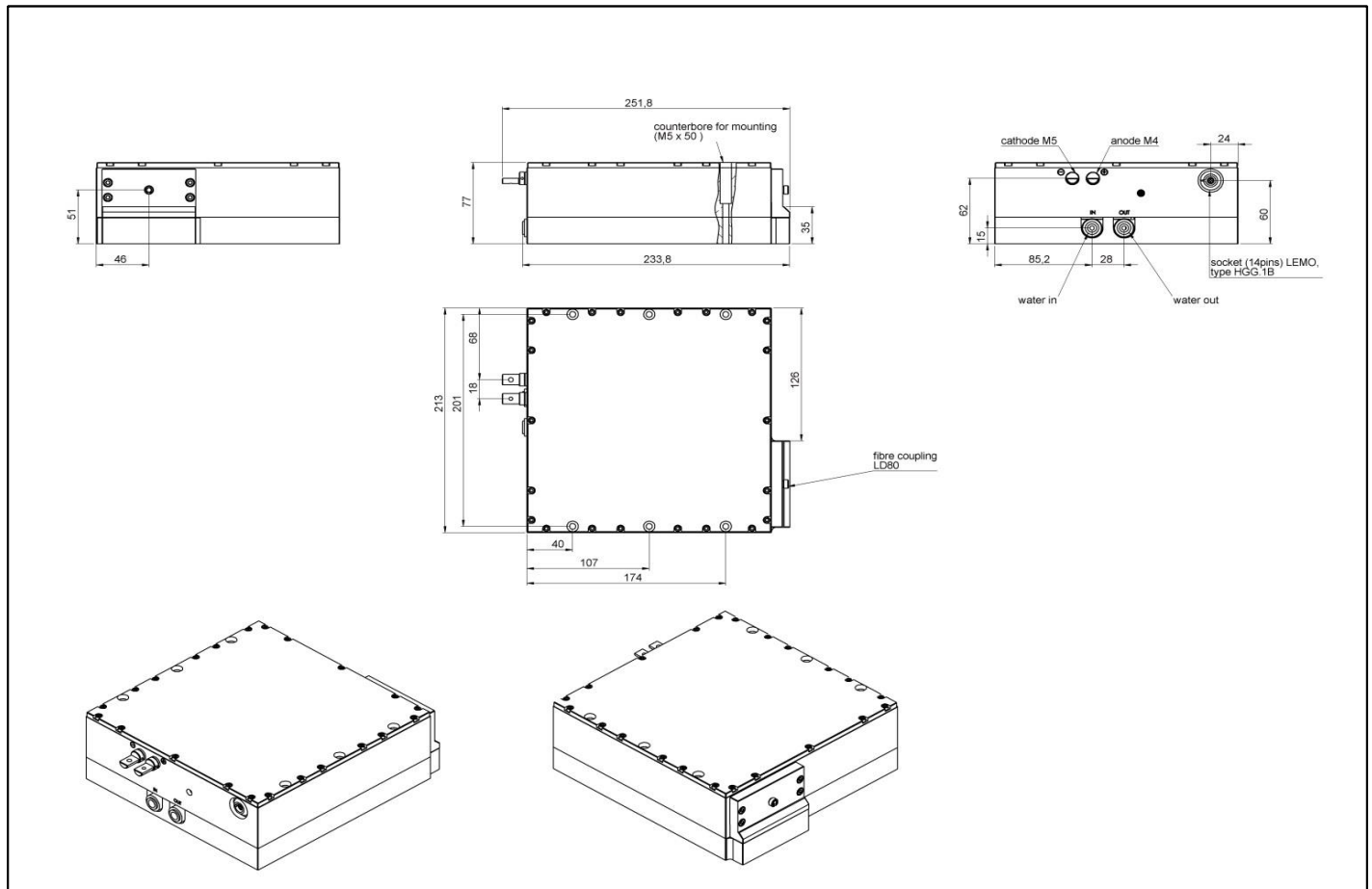
LIMO400-F400-DL980-S3012 prepared for water cooling
