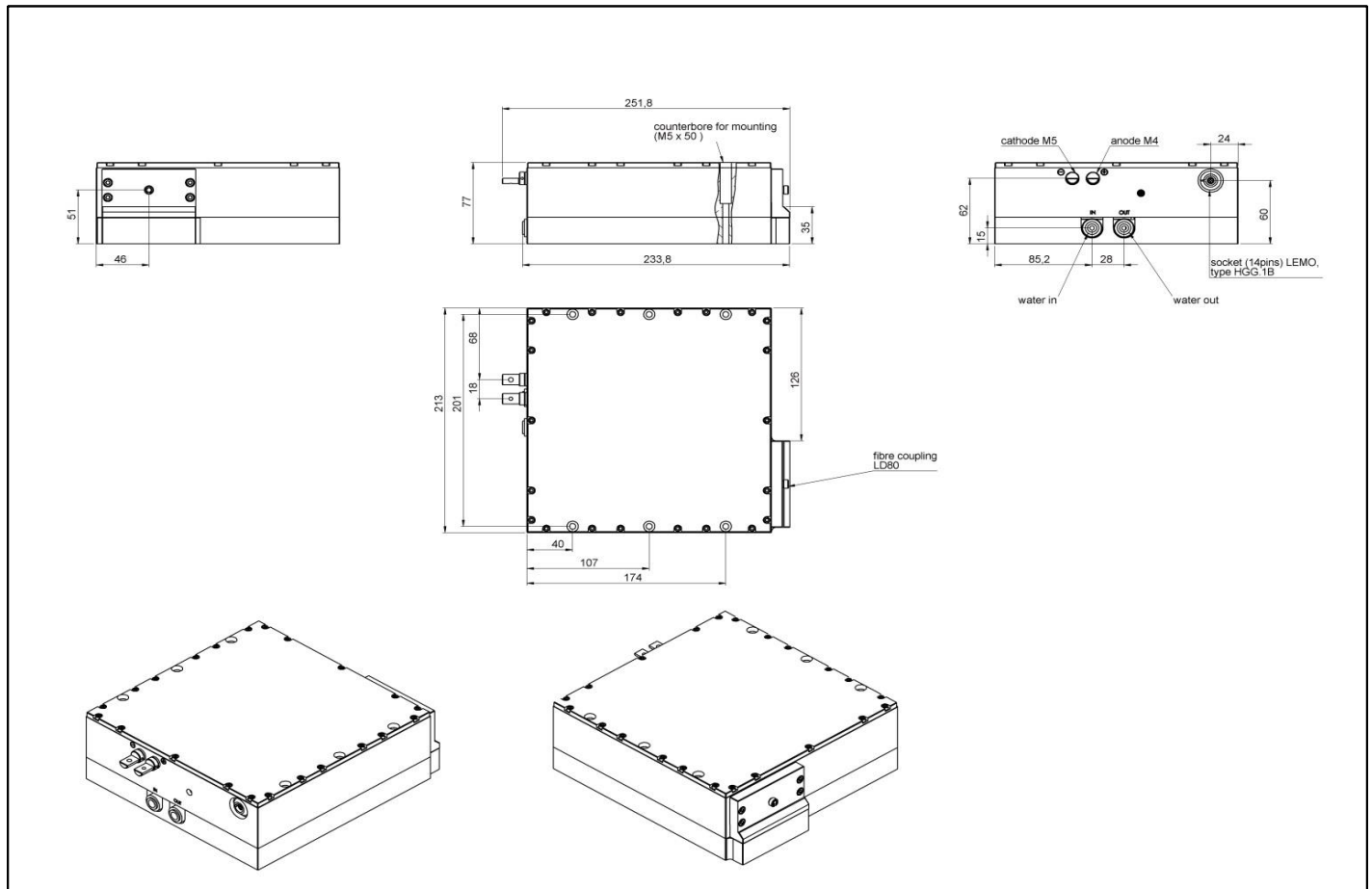
LIMO500-F400-DL980-S3013 prepared for water cooling
