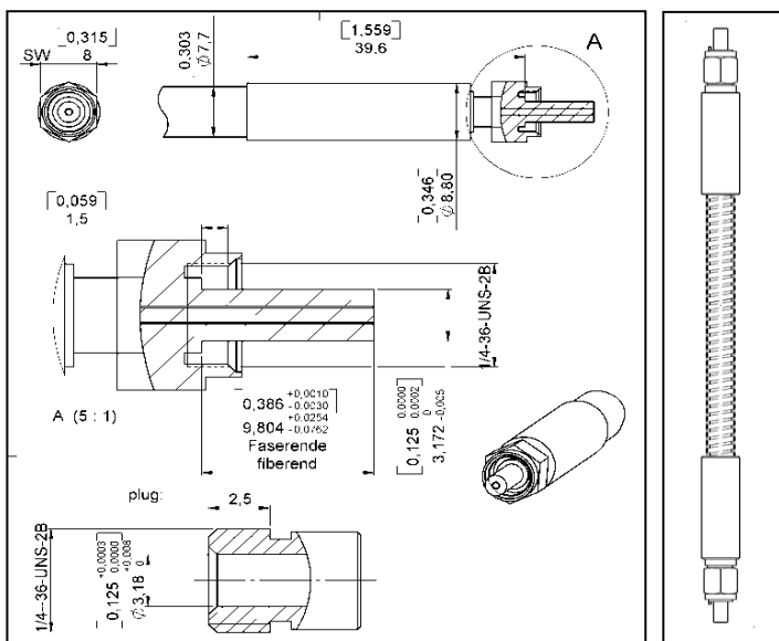
SMA Connector
